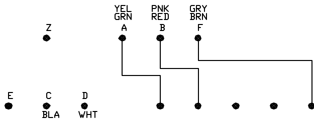
A 10 READER HEAD CABLE CONNECTIONS
